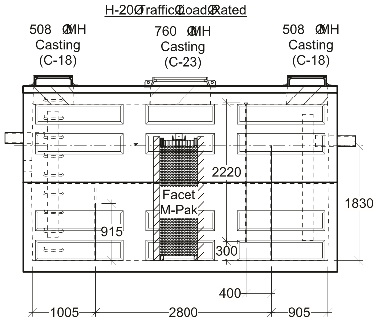
Side View
