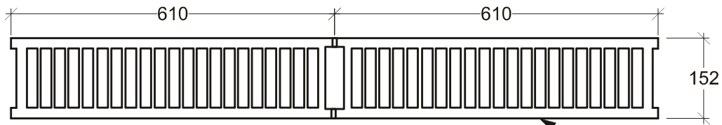
Plan View - Grate
