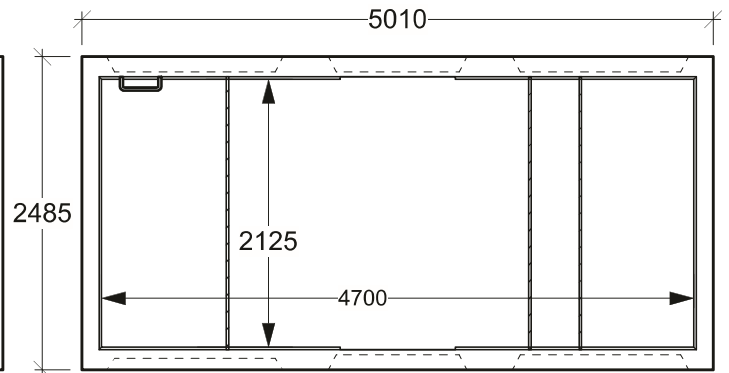
Plan View - Bottom
