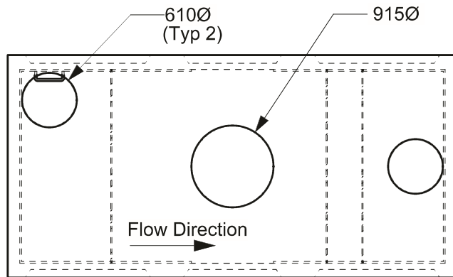
Plan View - Top
