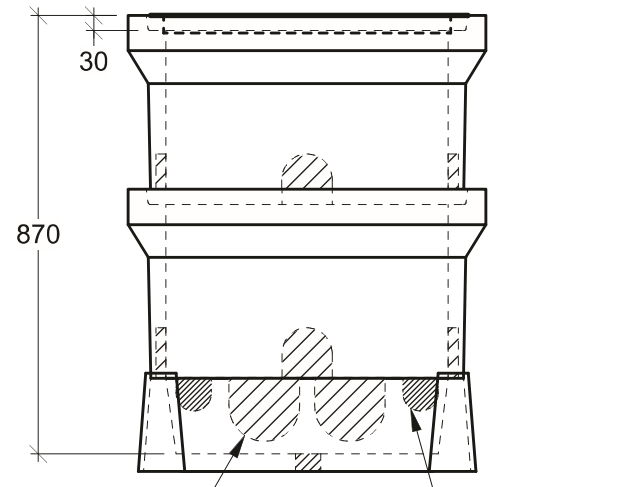
End View
