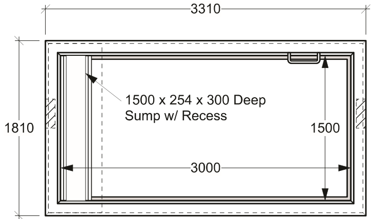
Plan View - Bottom
