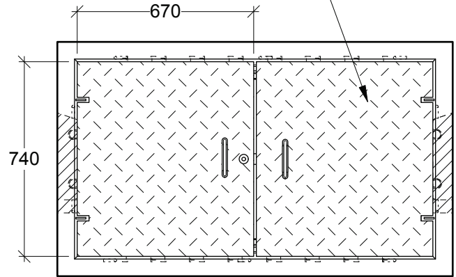
Plan View - Vault w/ Covers
