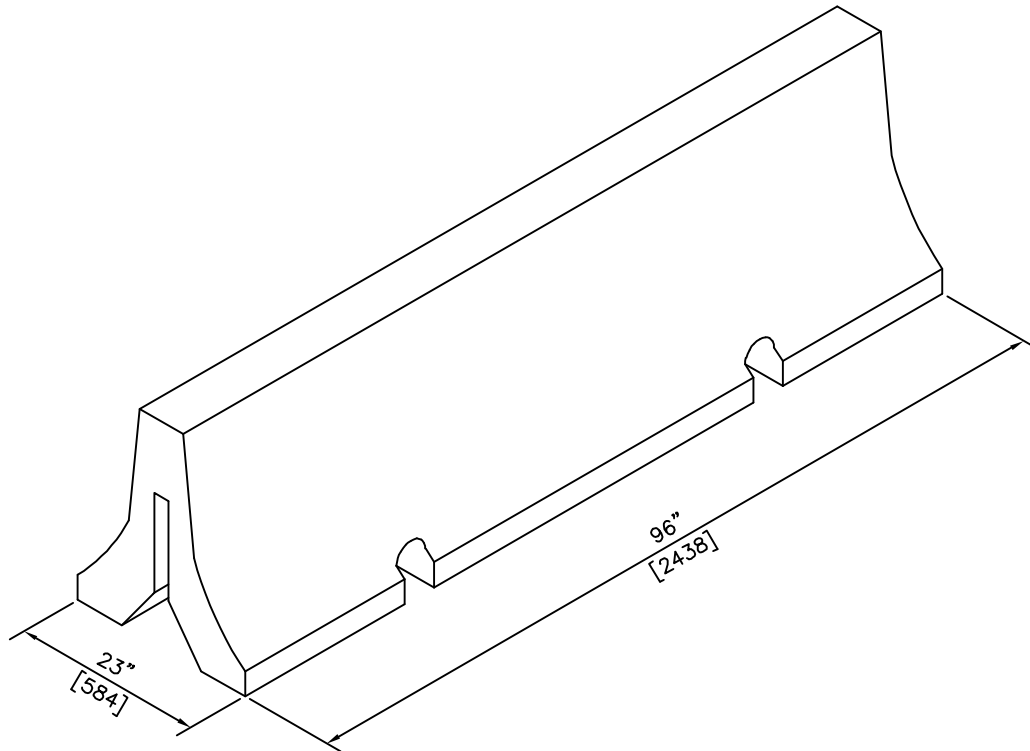
ISOMETRIC
